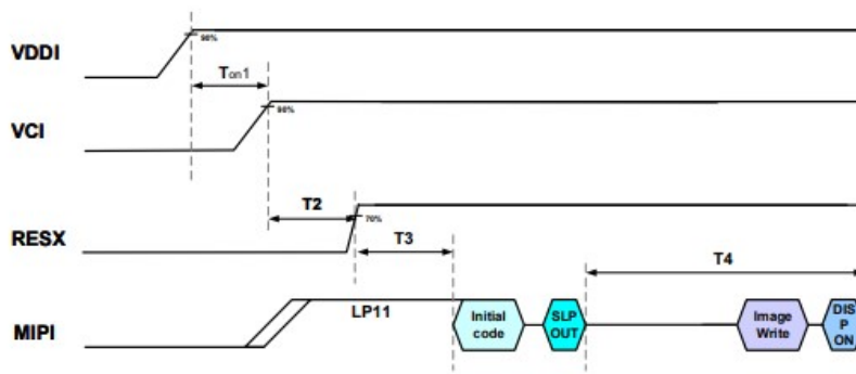
MIPI Power ON Sequence
